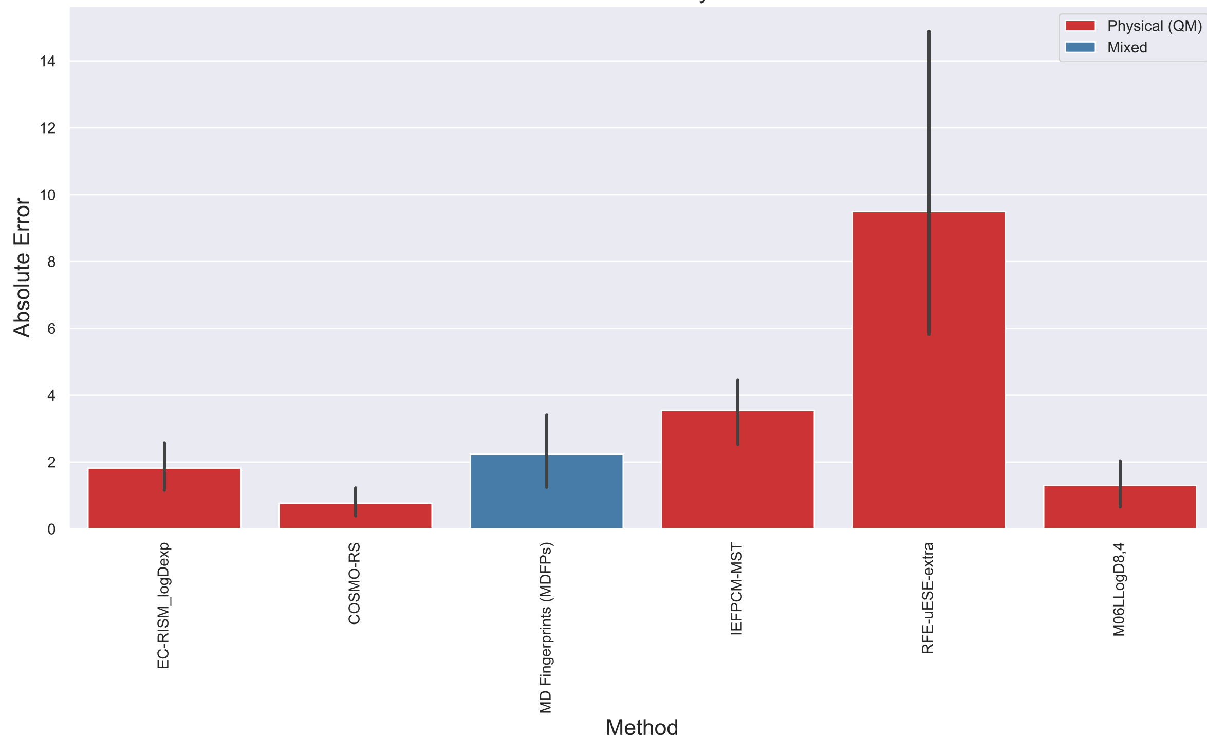
Absolute Error Plot for Ethyl acetate-water
